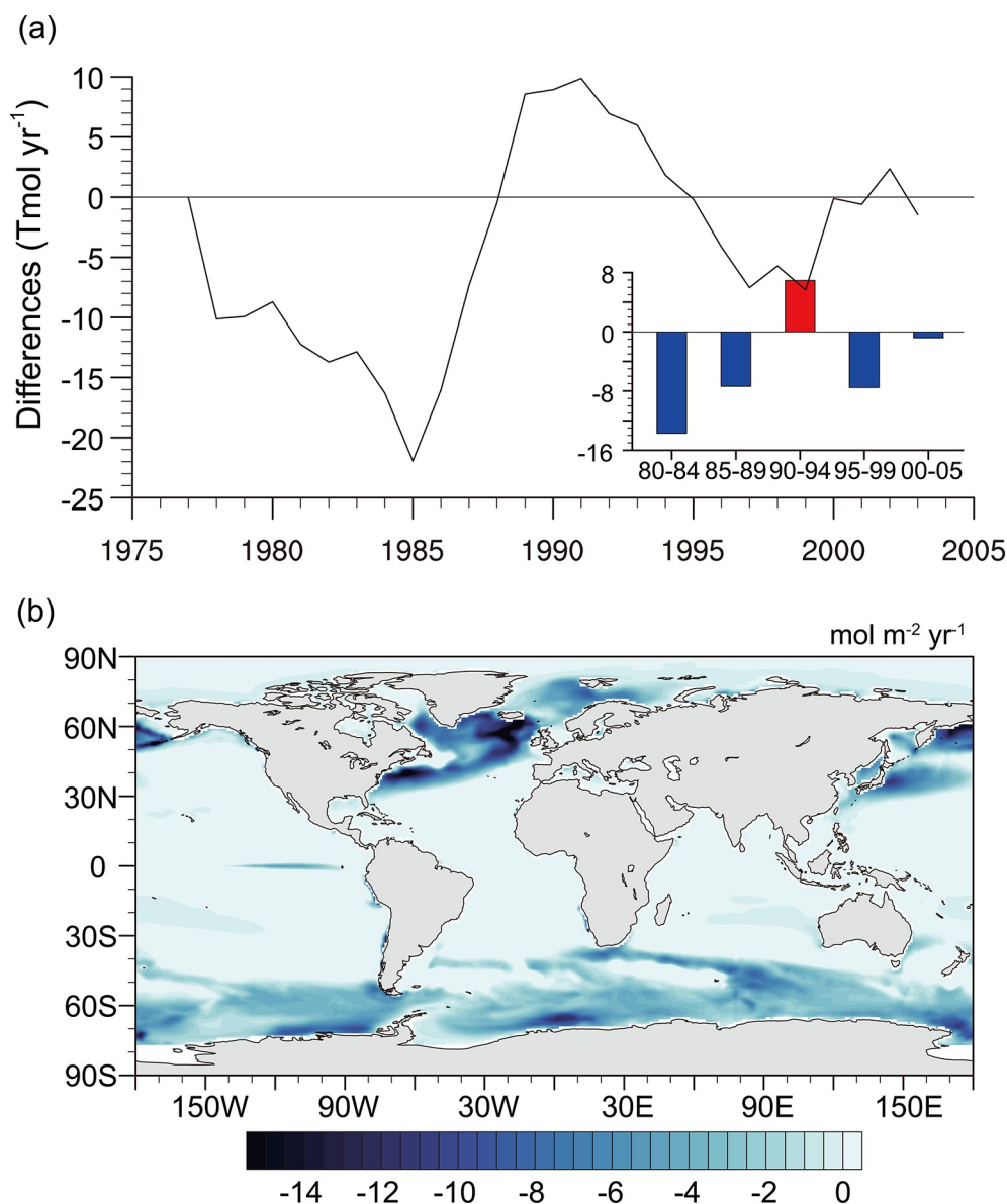
Fig. 5. Differences of air-sea O 2 flux between CMIP6 and CMIP5 during period 1975–2005 (i.e. FLUX_{CMIP6} minus FLUX_{CMIP5} ). The black line in (a) is the time series of the difference and (b) shows the spatial distribution of the difference averaged from 1975–2005.
