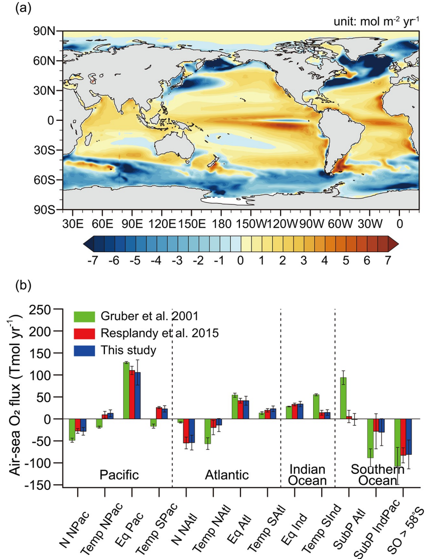
Fig. 1. The spatial distributions of annual mean air-sea O 2 flux (a) averaged from 1985 to 2014 in CMIP6 historical simulations, and (b) compared with two other studies. Positive flux in Fig. 1a means O 2 outgassing from ocean to the atmosphere. For sake of comparisons, the ocean is partitioned into 13 regions as shown in Fig. S3 in the ESM. The results from Li et al (2020) are similar with Resplandy et al 2015, which are not shown here.
