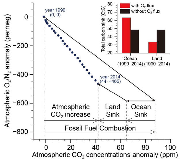
Fig. 8. Role of air-sea O 2 flux in O 2 -based carbon sinks estimations. The diagram is same as Fig. 6 , except for no air-sea O 2 flux considered in the calculation. The bar charts in the top right show the comparisons between estimated ocean/land carbon sink with and without O 2 flux correction.
