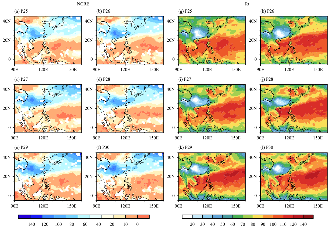
Fig. 4. Geographical distributions of (a–f) net cloud radiative effect (NCRE; \text{W m}^{-2} ) and (g–l) top-of-atmosphere radiation budget (TOA R_t ; \text{W m}^{-2} ) in pentads 25–30 during 2001–2016.
