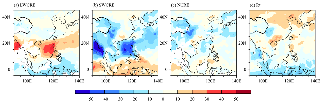
Fig. 5. Geographical distributions of the differences in (a) LWCRE ( \text{W m}^{-2} ), (b) SWCRE ( \text{W m}^{-2} ), (c) NCRE ( \text{W m}^{-2} ), and (d) R_t ( \text{W m}^{-2} ) between pentads 25–26 and 29–30 during 2001–2016.
