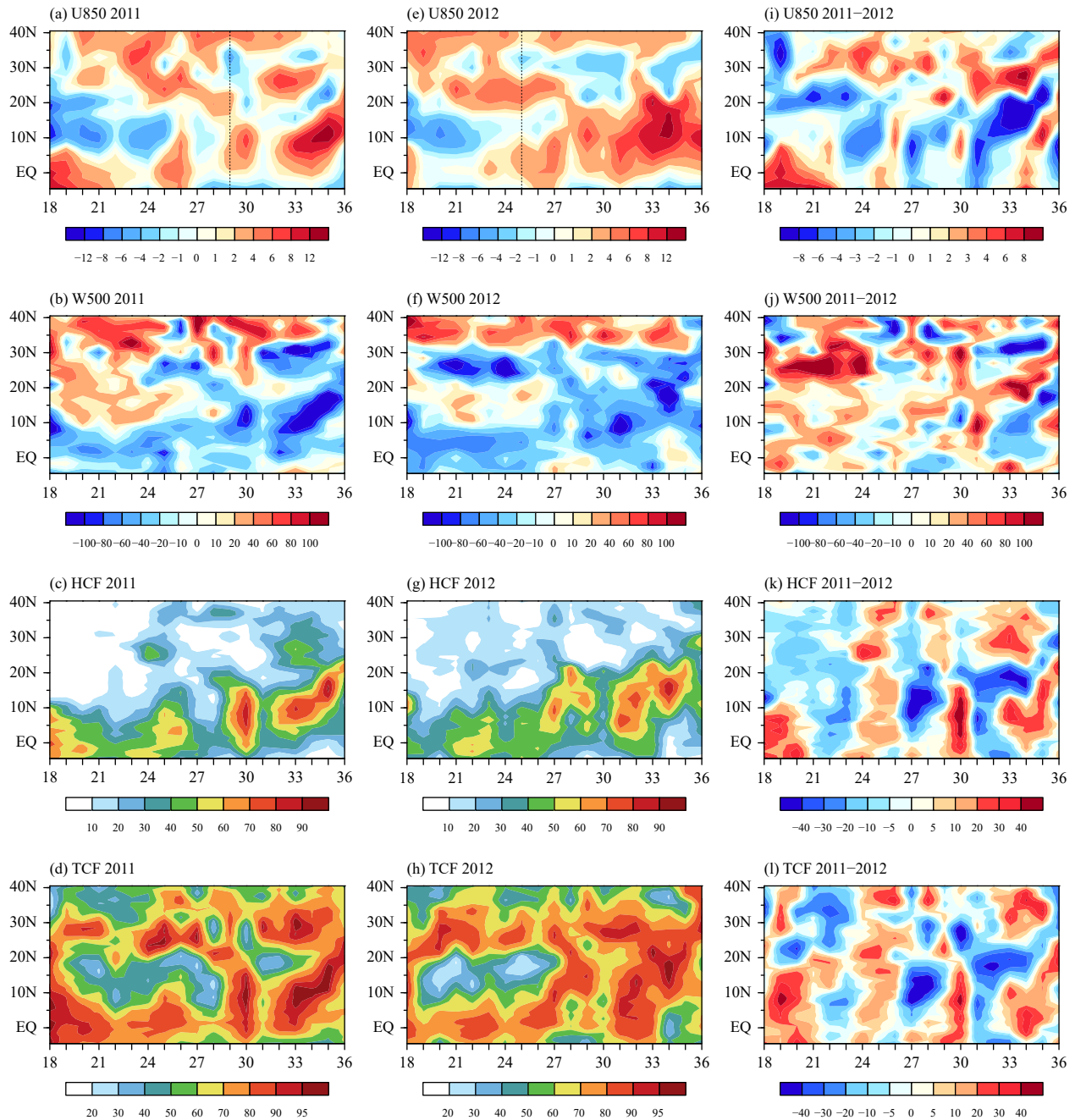
Fig. 8. Pentad mean changes in (a) 850-hPa zonal wind (U850; \text{m s}^{-1} ), (b) 500-hPa vertical velocity (W500; \text{hPa day}^{-1} ), (c) HCF (%), and (d) TCF (%) averaged over 110^{\circ} – 120^{\circ}\text{E} in pentads 18–36 of 2011; (e–h) the counterparts in 2012; and (i–l) the differences between 2011 and 2012. The x -axis denotes the pentad number. The black dashed lines in (a, e) denote the SCSSM onset pentad in 2011 and 2012.
